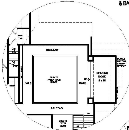
"OPTIONAL" BALCONY @ FAMILY ROOM w/ OPTIONAL READING NOOK
