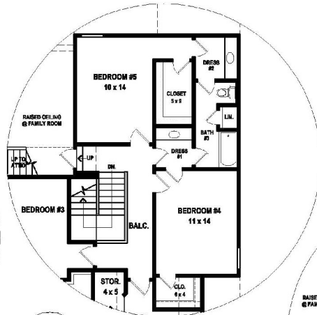
"OPTIONAL" BEDROOM #5 w/ JACK-N-JILL BATH
