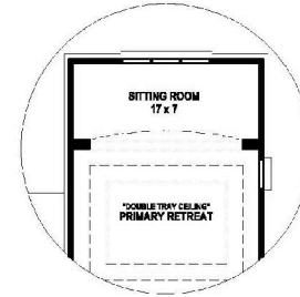
"OPTIONAL" SITTING ROOM
