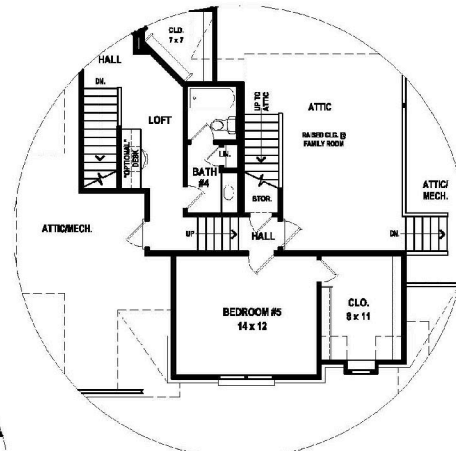
"OPTIONAL" SECOND FLOOR LAYOUT
