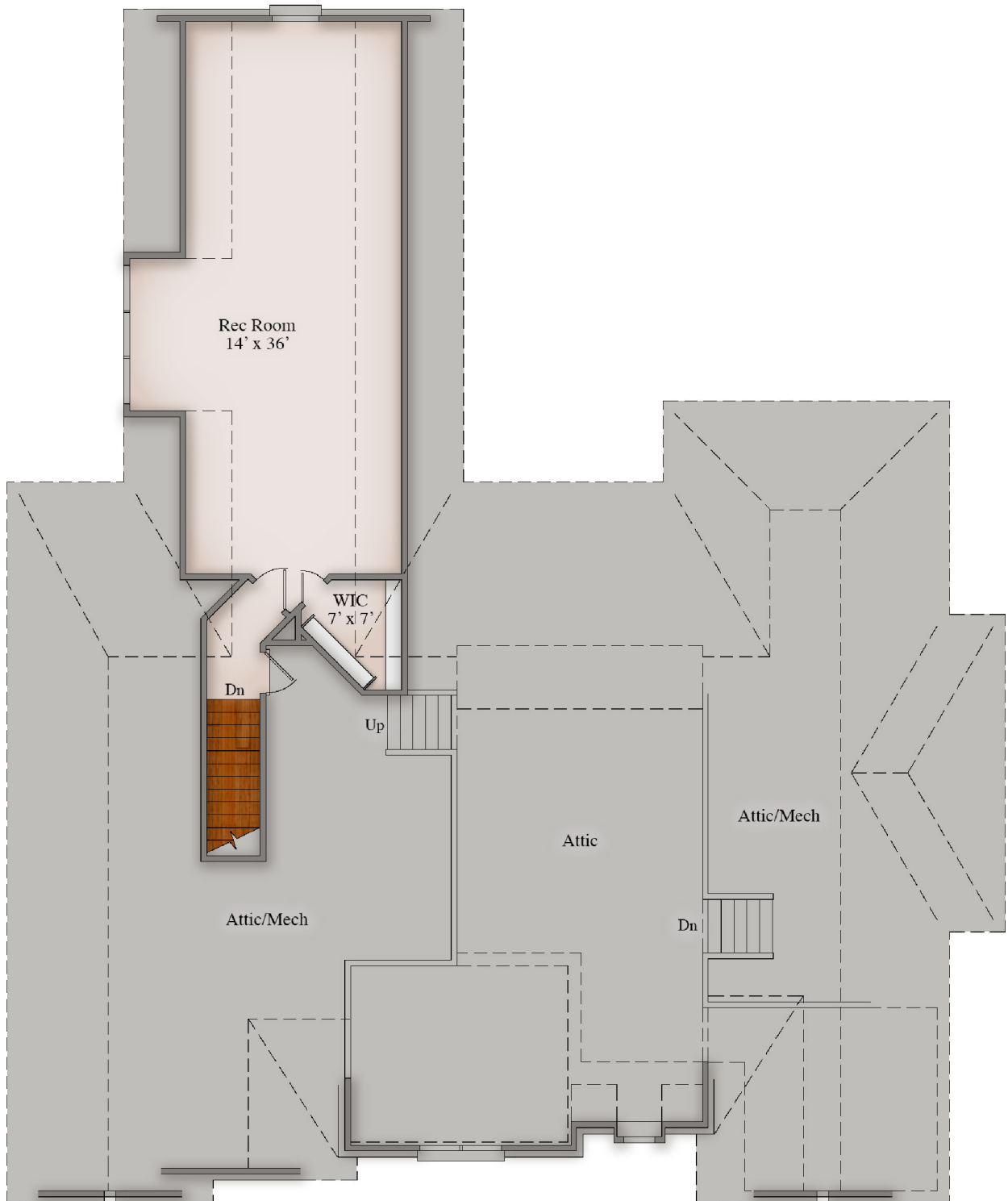
Second Floor: 9' Ceilings unless noted
