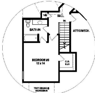
"OPTIONAL" BEDROOM #5 & BATH #4
