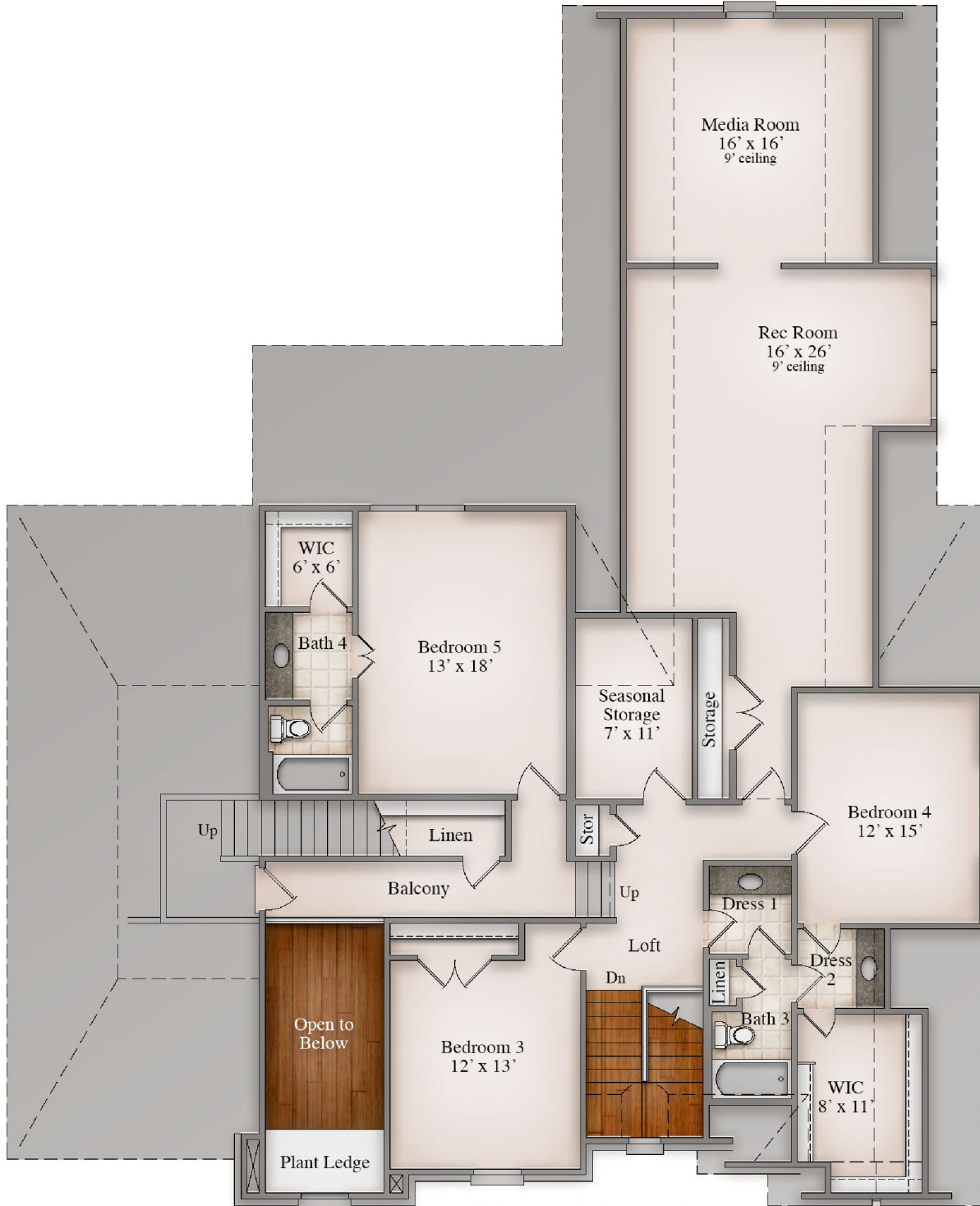
Second Floor: 9' Ceilings unless noted
